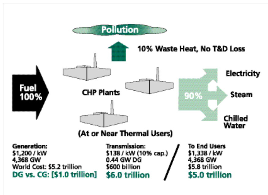
Figure 10. Combined heat and power flowchart
