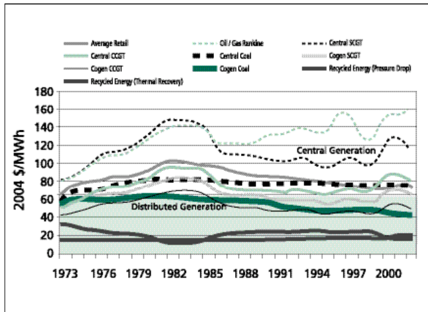
Figure 3. Long-term U.S. marginal cost of electric generation options
