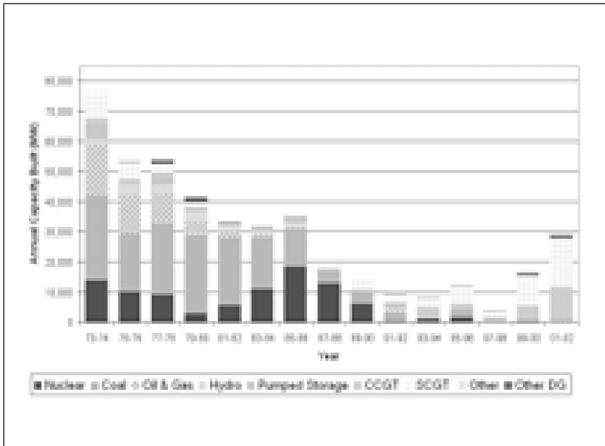
Figure 4. Annual U.S. utility additions of electricity generating capacity by technology, 1973–2002
