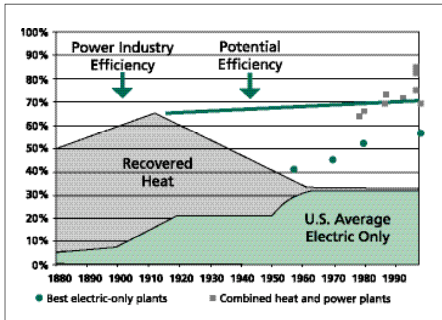
Figure 2. U.S. electricity generating efficiency, 1880 to present
